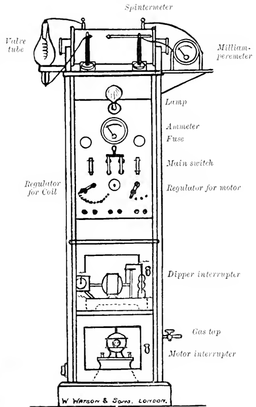
FIG. 79.—To illustrate the parts as arranged in Fig. 78.
